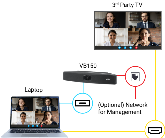
Two Cable BYOD
